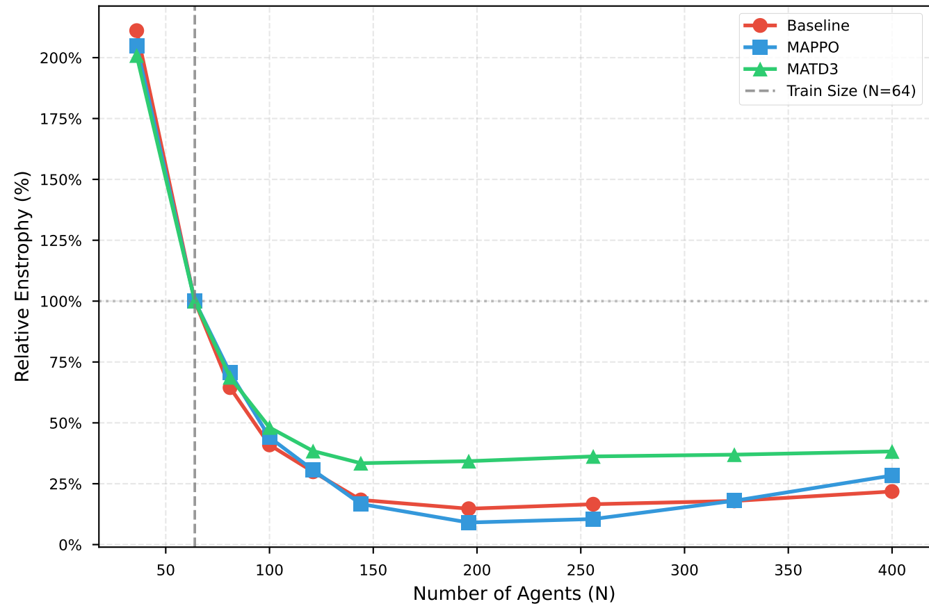
Relative Scalability (Zero-Shot)
