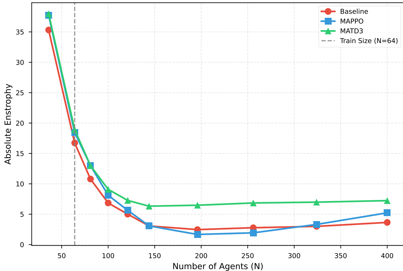
Absolute Scalability (Zero-Shot)
